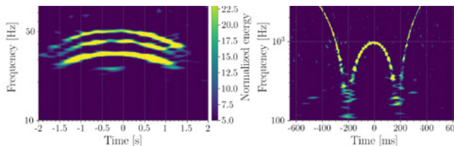
Time-frequency depictions of transient noise from Advanced LIGO's second observing run. Left: Arches caused by scattered light recombining with the main laser. Right: A whistle caused by beatnotes between drifting RF oscillators.
