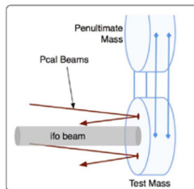
Figure 3: The photon calibrator system.
